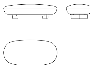
52570 Pouf con base in frassino Stool with base in ash wood cm 157 x 76 x h 44 in 61 7/8 x 30 x h 17 3/8
