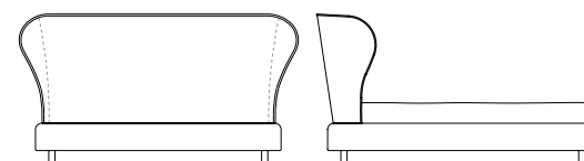
*SF 51971 + 51970 Giroletto imbottito + Testata Upholstered base + Headboard cm 225 x 227 x h 120 in 88 1/2 x 89 3/8 x h 47 1/4 RETE - SLAT BASE cm 180 in 70 7/8
